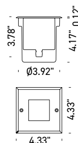
Fixture Dimensions
