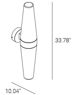
Fixture Dimensions
