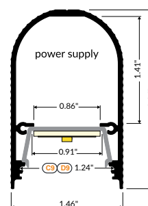
Fixture Dimensions
