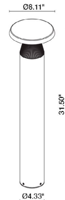
Fixture Dimensions
