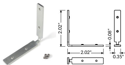
V5999519S Connector Q9 1 90° Bent Zinc Coated Steel
