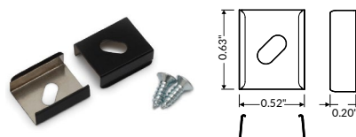
892700__ Mounting Plate Z
