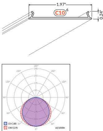
P2001438 - 78.7 in P2001638 - 157.5 in Diffuser C10 6 click Basic
