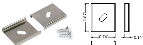
A2090019 Mounting Plate Y Inox Stainless Steel
