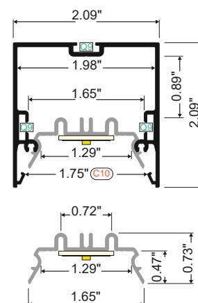
Fixture Dimensions
