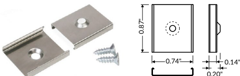
A2130019 Mounting Plate Y Cone Inox Stainless Steel
