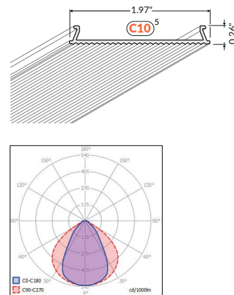
P2001016 - 78.7 in P2001216 - 159.5 in Diffuser C10 5 click Pro
