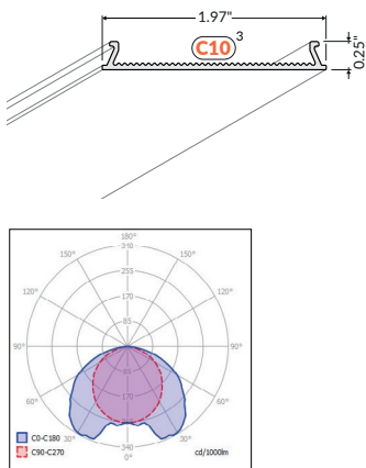
63590000 - 78.7 in 63780000 - 157.5 in Diffuser C10 3 click Wide
