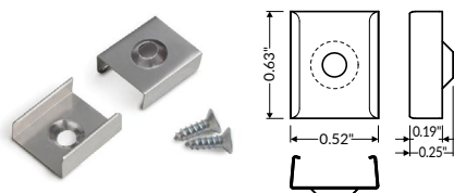
899800__ Mounting Plate Z Cone
