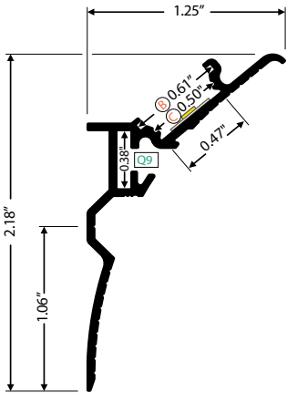
Fixture Dimensions
