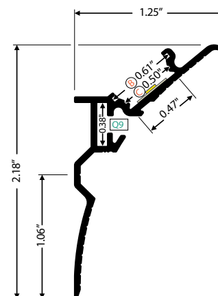
Fixture Dimensions
