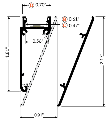
Fixture Dimensions
