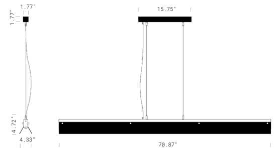
Fixture Dimensions
