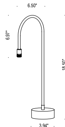
Fixture Dimensions
