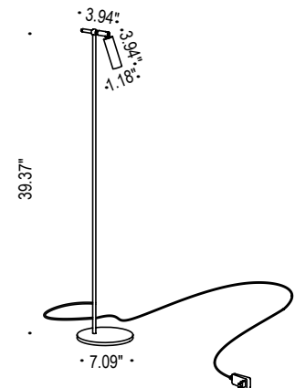
Fixture Dimensions
