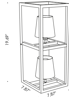
Fixture Dimensions
