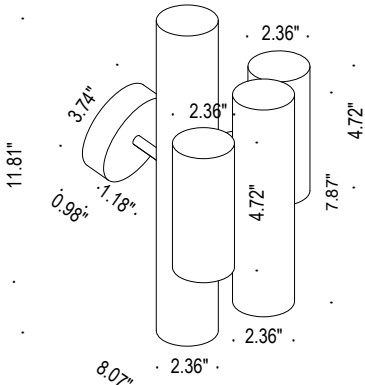
Fixture Dimensions
