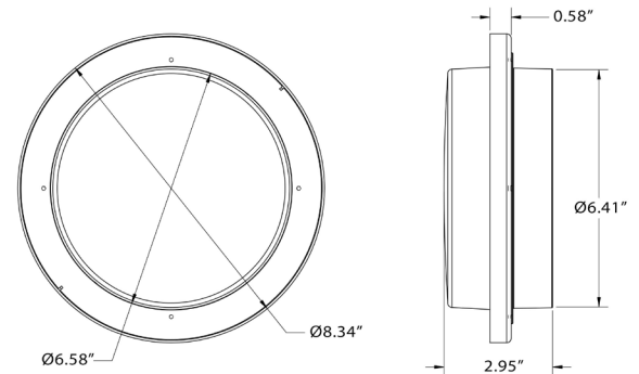
Fixture Dimensions
