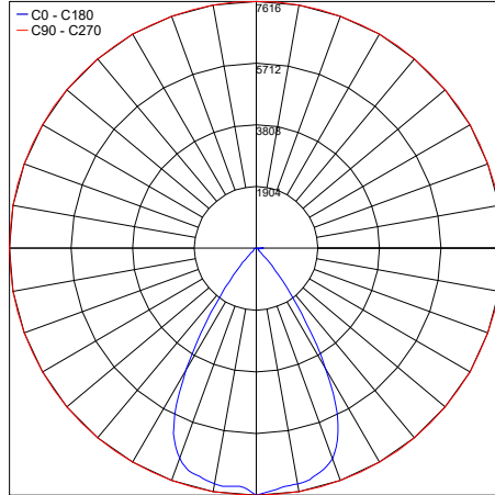
PHOTOMETRIC FILENAME : BAJA C-300 R 30K 10x45° - PT9022032N.IES
