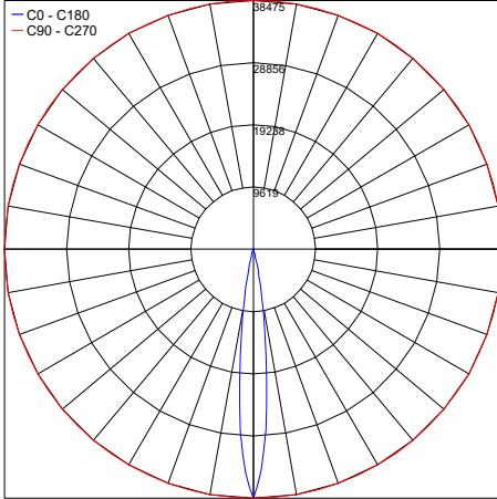
PHOTOMETRIC FILENAME : BAJA C-300 R 30K 10° - PT9022031N.IES
