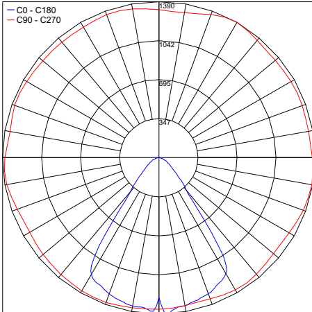
PHOTOMETRIC FILENAME : BAJA C-300 R 30K 70° - PT9022037N.IES
