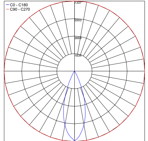
PHOTOMETRIC FILENAME : BAJA C-300 R 30K 45° - PT9022034N.IES
