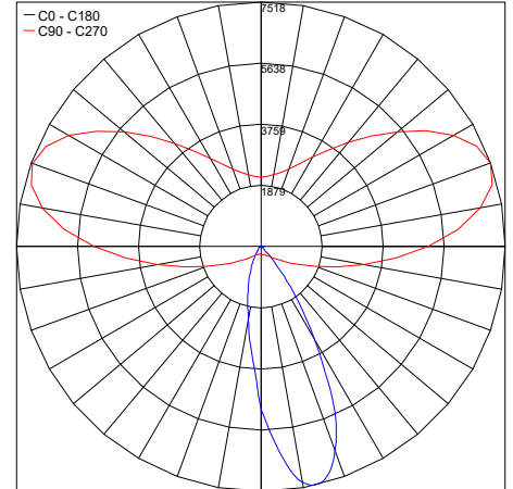
PHOTOMETRIC FILENAME : BAJA C-300 R 30K ASYM WIDE - PT9022038N.IES
