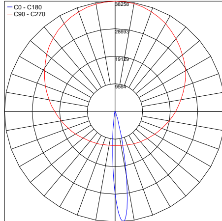
PHOTOMETRIC FILENAME : BAJA C-300 R 30K ASYM NARROW - PT9022039N.IES
