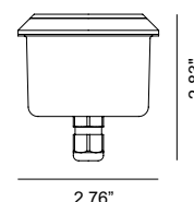
Fixture Dimensions
