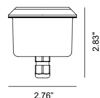
Fixture Dimensions
