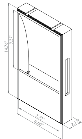
Fixture Dimensions
