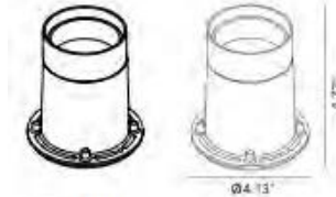
PT51900 Casing F80 H120 4.13" w x 4.72" h
