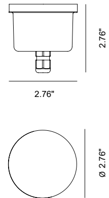
Fixture Dimensions
