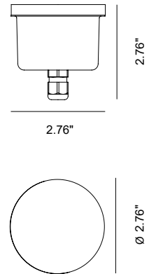
Fixture Dimensions
