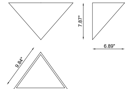
Fixture Dimensions:
