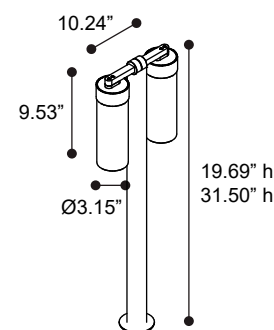
Fixture Dimensions
