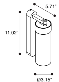
Fixture Dimensions
