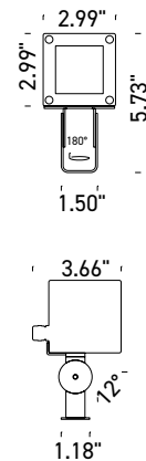
Fixture Dimensions
