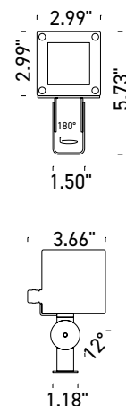
Fixture Dimensions
