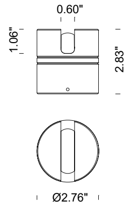
Fixture Dimensions
