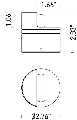
Fixture Dimensions
