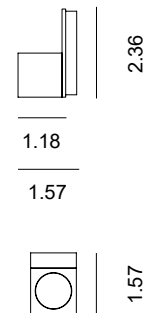
Fixture Dimensions
