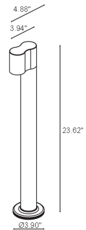
Fixture Dimensions
