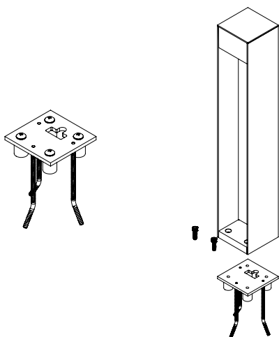
AM-00017 Mounting Base Assembly
