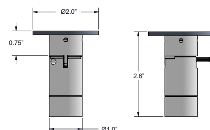
Fixture Dimensions
