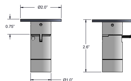
Fixture Dimensions
