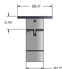
Fixture Dimensions
