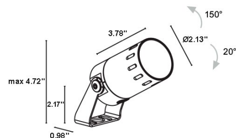
Fixture Dimensions
