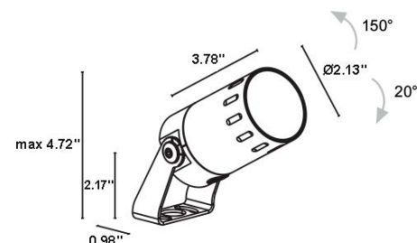
Fixture Dimensions
