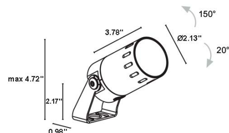
Fixture Dimensions
