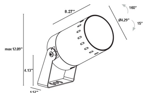
Fixture Dimensions
