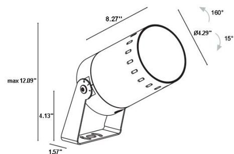
Fixture Dimensions
