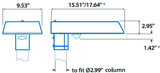
Vertical Column Top 55W Versions
