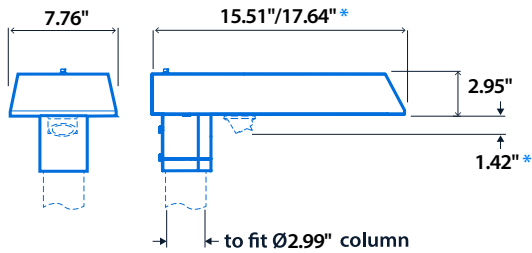
Vertical Column Top 9W / 27W Versions
