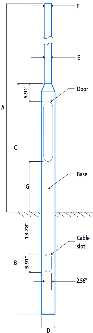
Acorn Column See Table for varying dimensions.
