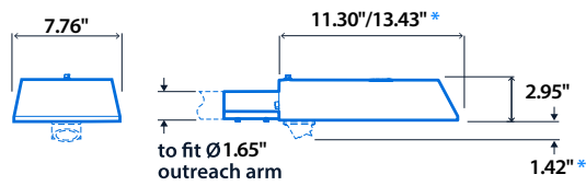
Horizontal Outreach Arm 9W / 27W Versions
