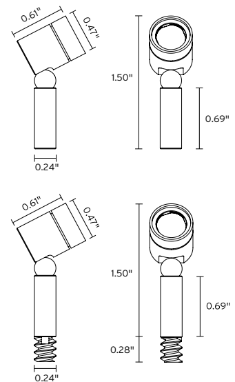
Fixture Dimensions
