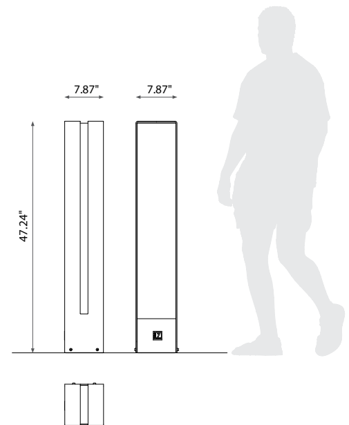
Fixture Dimensions
