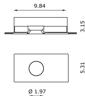
Fixture Dimensions
