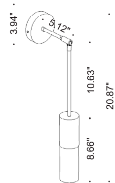
Fixture Dimensions
