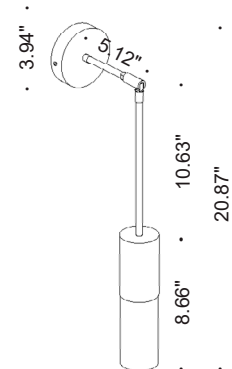
Fixture Dimensions
