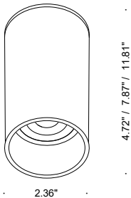
Fixture dimensions
