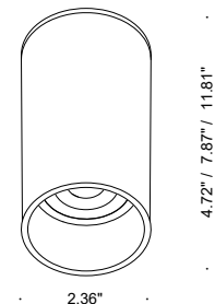
Fixture dimensions
