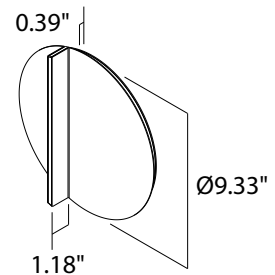
Fixture Dimensions
