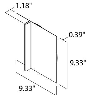
Fixture Dimensions
