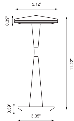
Fixture Dimensions
